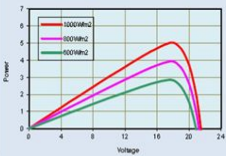
Power-Voltage Relationship, variable light intensity
